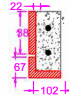
Structural Reinforced Concrete Backing
