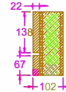
Non-Structural cement particle board with Polytherane core
