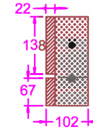
Non-Structural Lightweight Concrete
